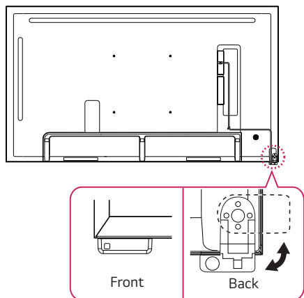
Horizontal Use (Default Mount)
